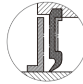
B-type Seal
