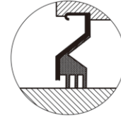
L3-type Seal
